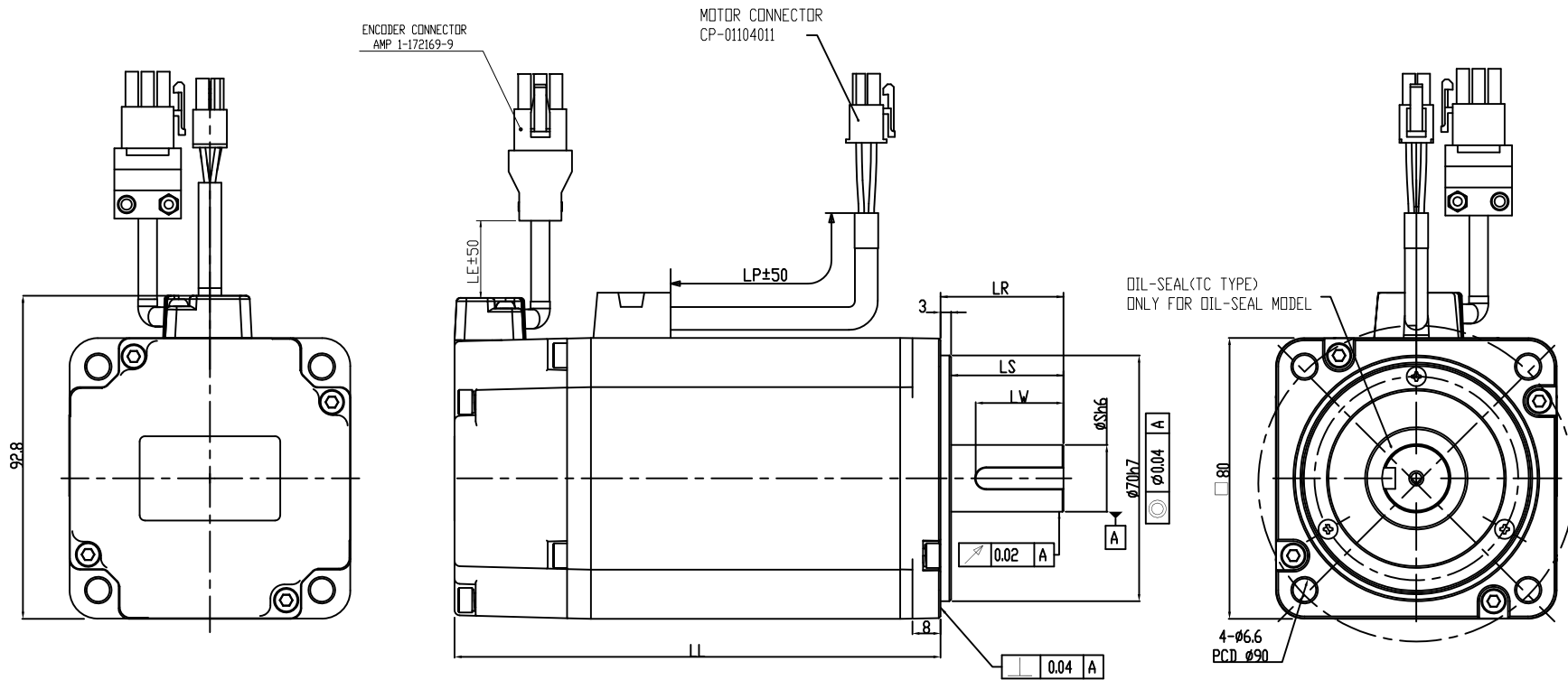
DIMENSION TABLE(MODEL WITHOUT BRAKE)
